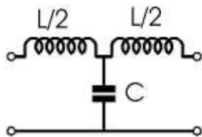
T section filter
