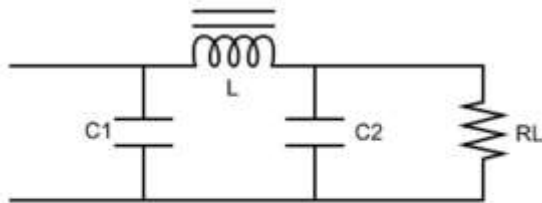
Pi Filter
